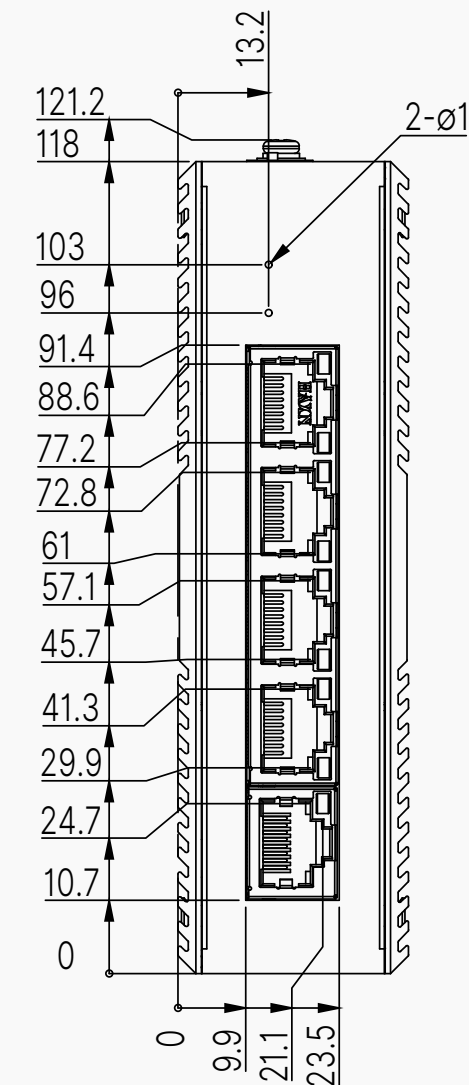
FRONT VIEW
